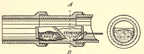
FIG. 10.—INVERT-FORMER.
